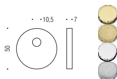
PB13/05 MOSTRINA TONDA PER CILINDRO CON POMOLO ROUND BACKPLATE FOR CYLINDER WITH KNOB
