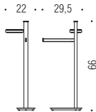
B9102S Piantana con porta sapone e porta salvietta Floor standing column with soap holder and towel holder
