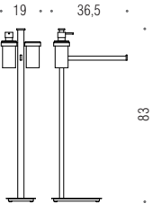
B9111 Piantana con spandisapone (L 0,28) porta bicchiere e porta salvietta Floor standing column with soap dispenser, glass holder and towel holder
