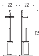
B9816 Piantana con porta rotolo e porta scopino sospeso in vetro acidato Floor standing column with paper holder and suspended acid glass brush holder
