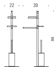
B9833 Piantana con porta salvietta, porta sapone, porta rotolo e porta scopino in ottone Floor standing column with towel holder, soap holder, paper holder and brass brush holder
