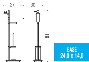
B9918 Piantana con spandisapone (L 0,15), porta salvietta, porta rotolo e porta scopino sospeso in vetro acidato Floor standing column with soap dispenser, towel holder, paper holder and suspended acid glass brush holder
