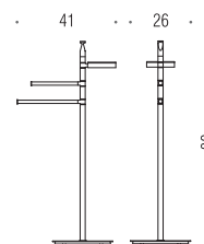
B9814 Piantana con porta sapone e 2 porta salvietta Floor standing column with soap holder and 2 towel holders
