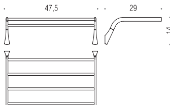
B2887 Rack porta salvietta Rack towel holder
