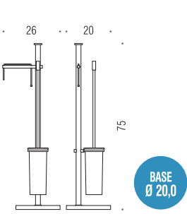
W4935 Piantana con porta rotolo e porta scopino Standing column equipped with paper holder and brush holder
