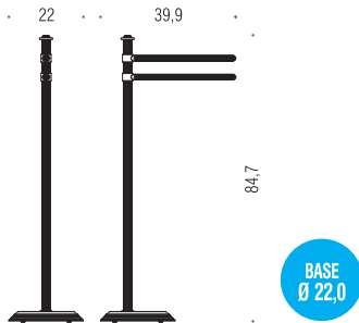
B3338 Piantana con due porta salvietta Standing column with two towel holders
