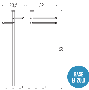
W4936 Piantana con due porta salvietta Standing column equipped with two towel holders
