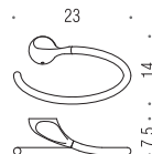
B1231 Porta salvietta ad anello Ring towel holder
